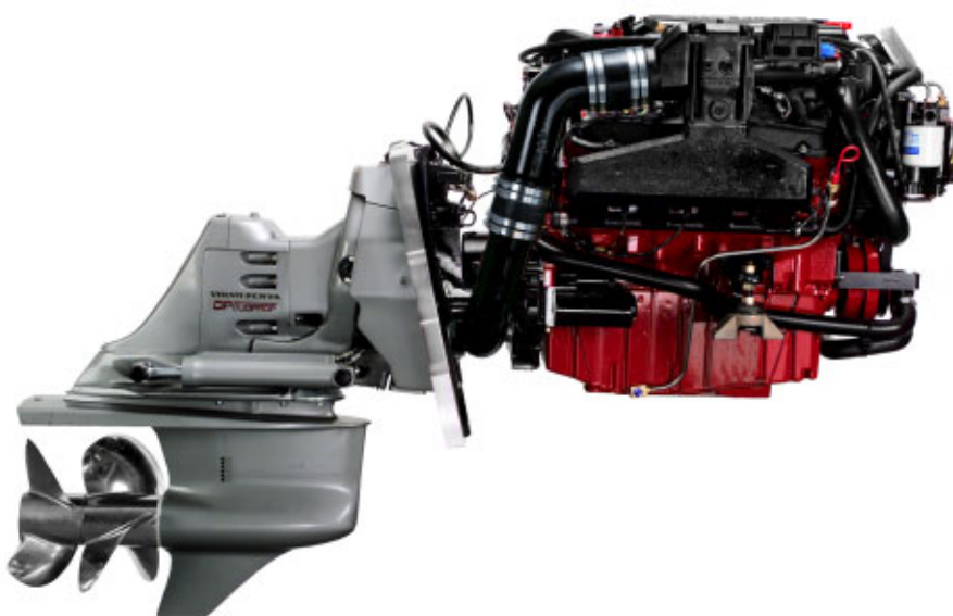
8.1GX i with DP-S Duoprop drive
